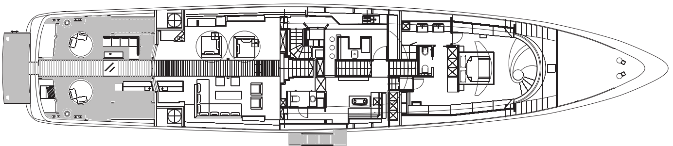
Main Deck
