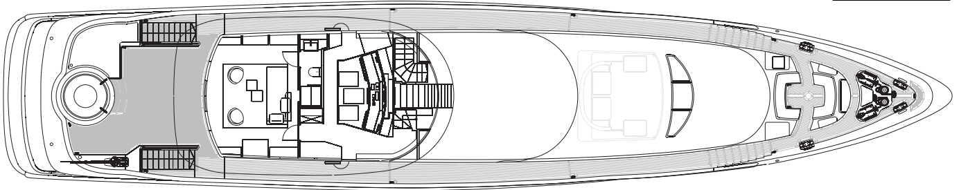
Upper Deck
