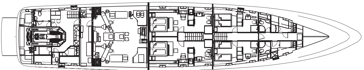
Lower Deck
