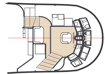
PILOTHOUSE
