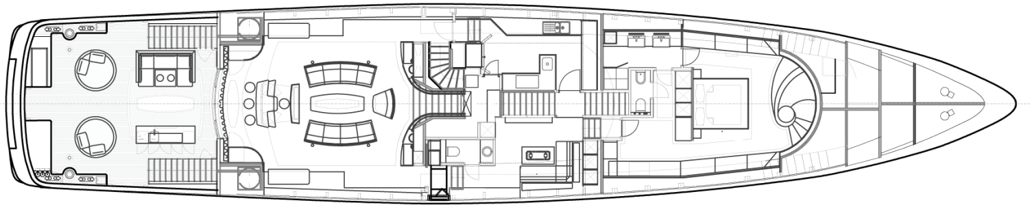
MAIN DECK
